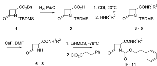
Scheme 1. Synthesis of 4-(alkylamino)carbonyl-1-phenethyloxy-carbonyl-2-azetidinones.
