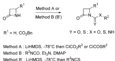
Scheme 2. Synthesis of N1-substituted \beta -lactams with ester, thioester, amide and thioamide groups.
